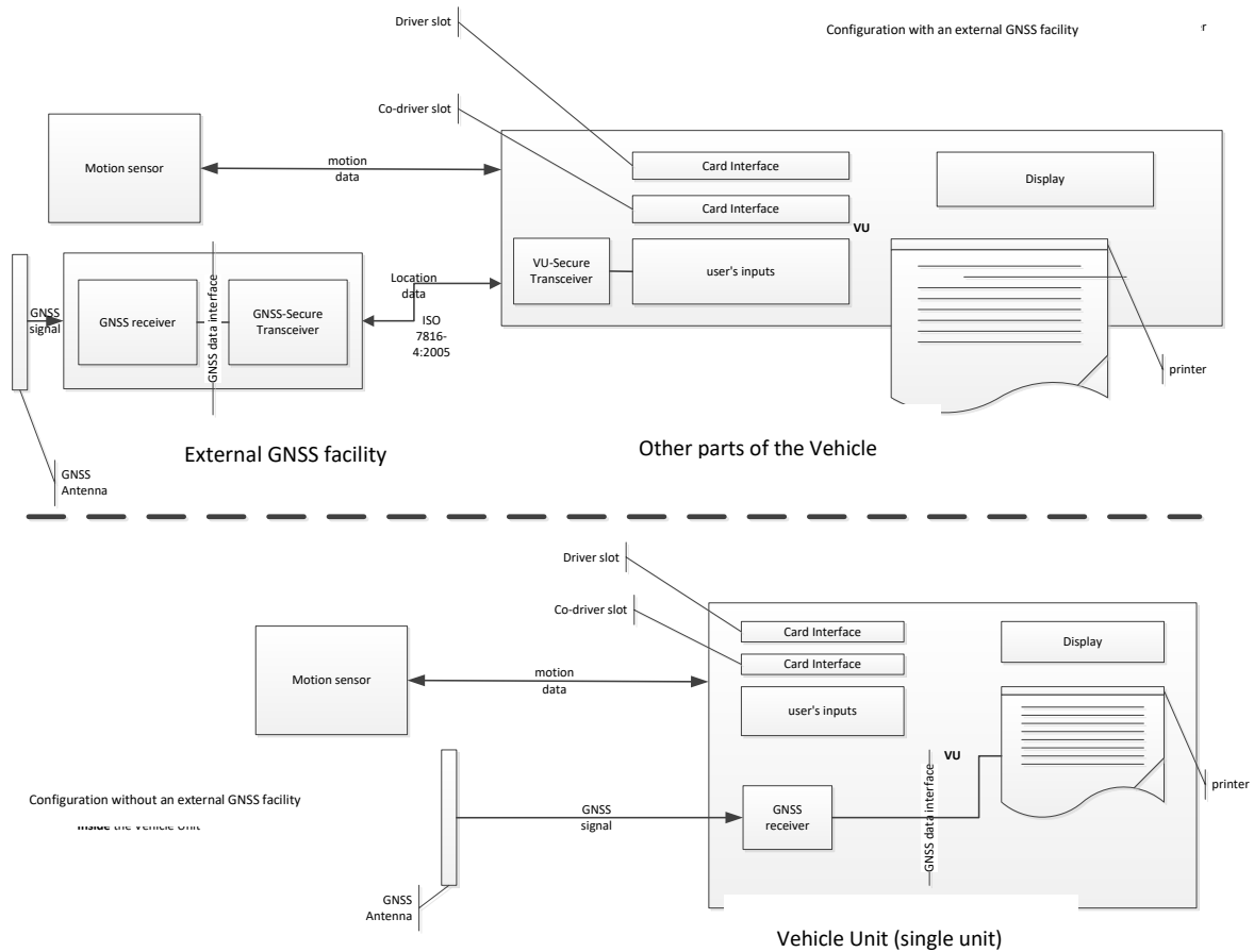
Figure 14 Different configurations for GNSS receiver.
