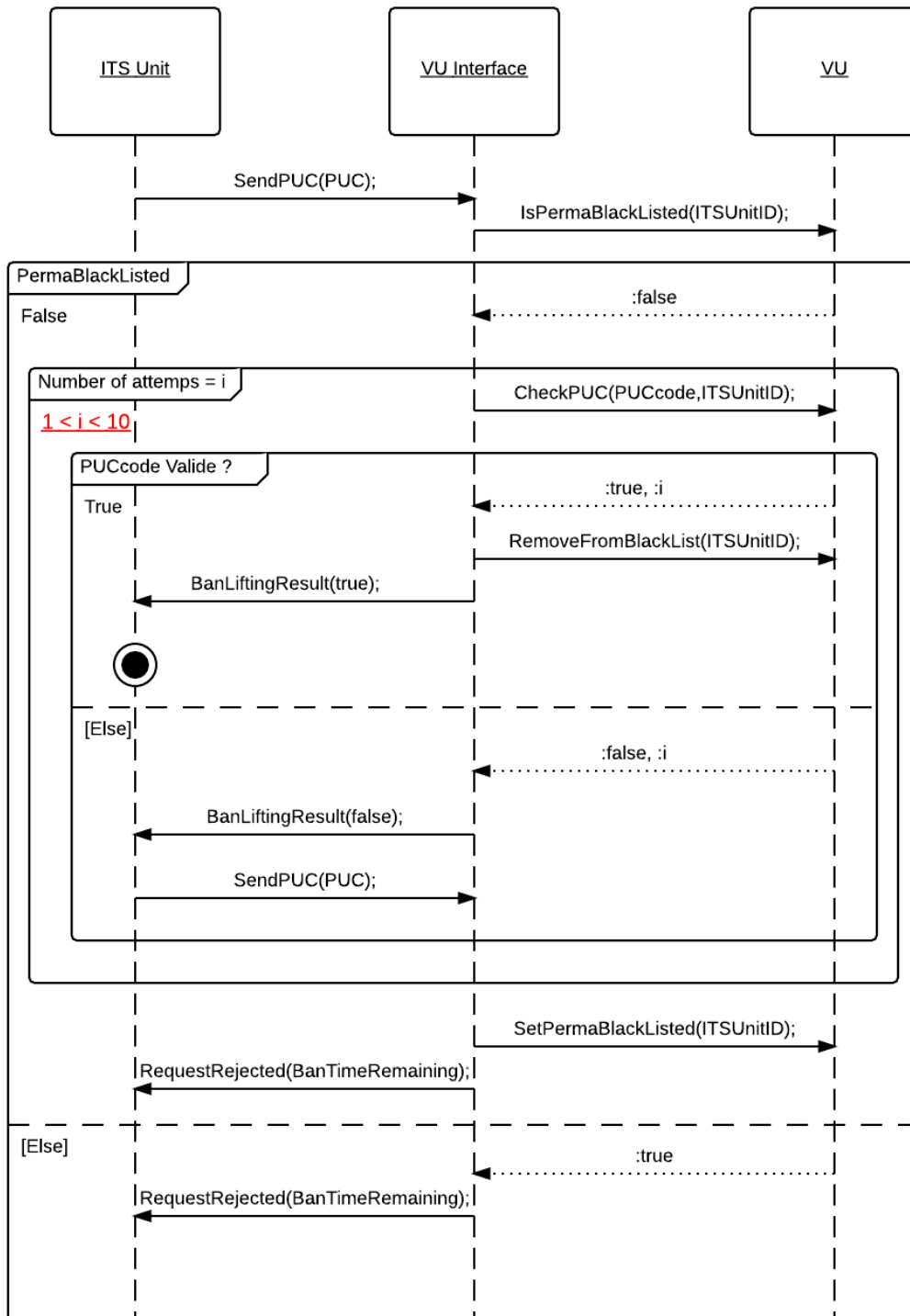
Figure 22. Sequence Diagram for PUC validation attempt
