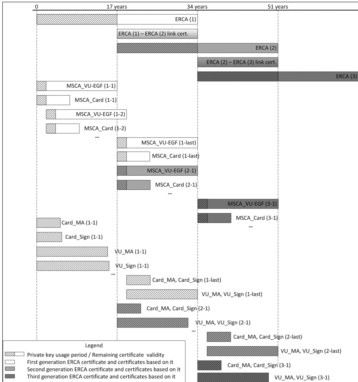
Figure 1 Issuance and usage of different generations of ERCA root certificates, ERCA link certificates, MSCA certificates and equipment certificates
