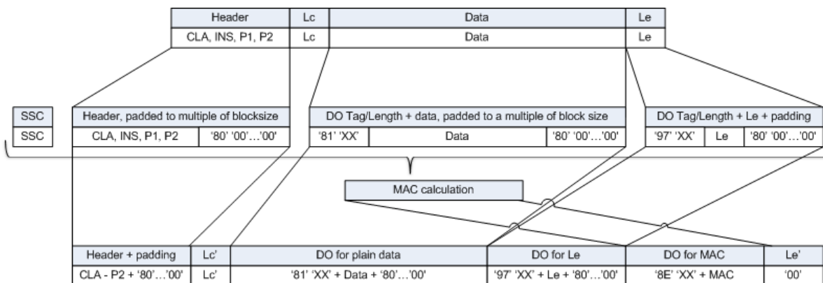
Figure 8 Transformation of an authenticated Case 4 Command APDU
