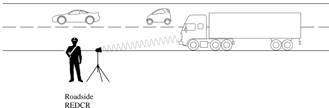
Figure 14.1 — Roadside interrogation using 5.8 GHz DSRC
