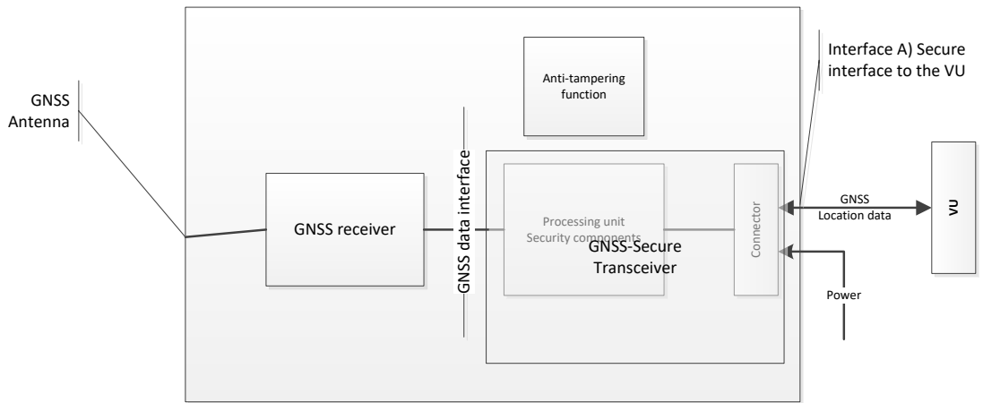
Figure 17 Schema of the external GNSS facility
