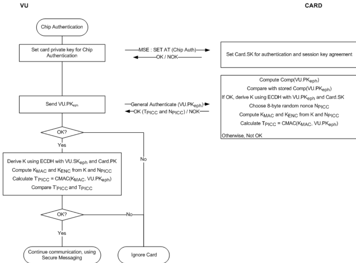
Figure 7 Chip Authentication and session key agreement
