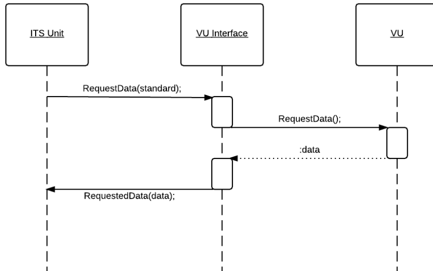
Figure 20. Sequence Diagram to process a request for data classified as non-personal (after correct PIN access)
