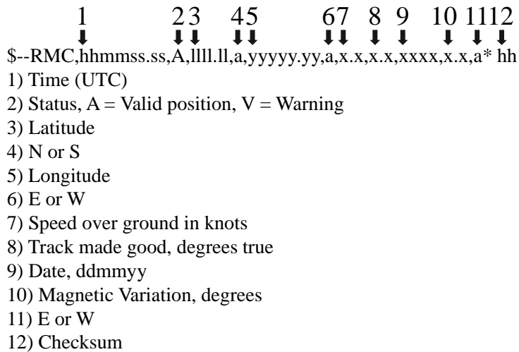
Figure 15 Structure of the RMC sentence
