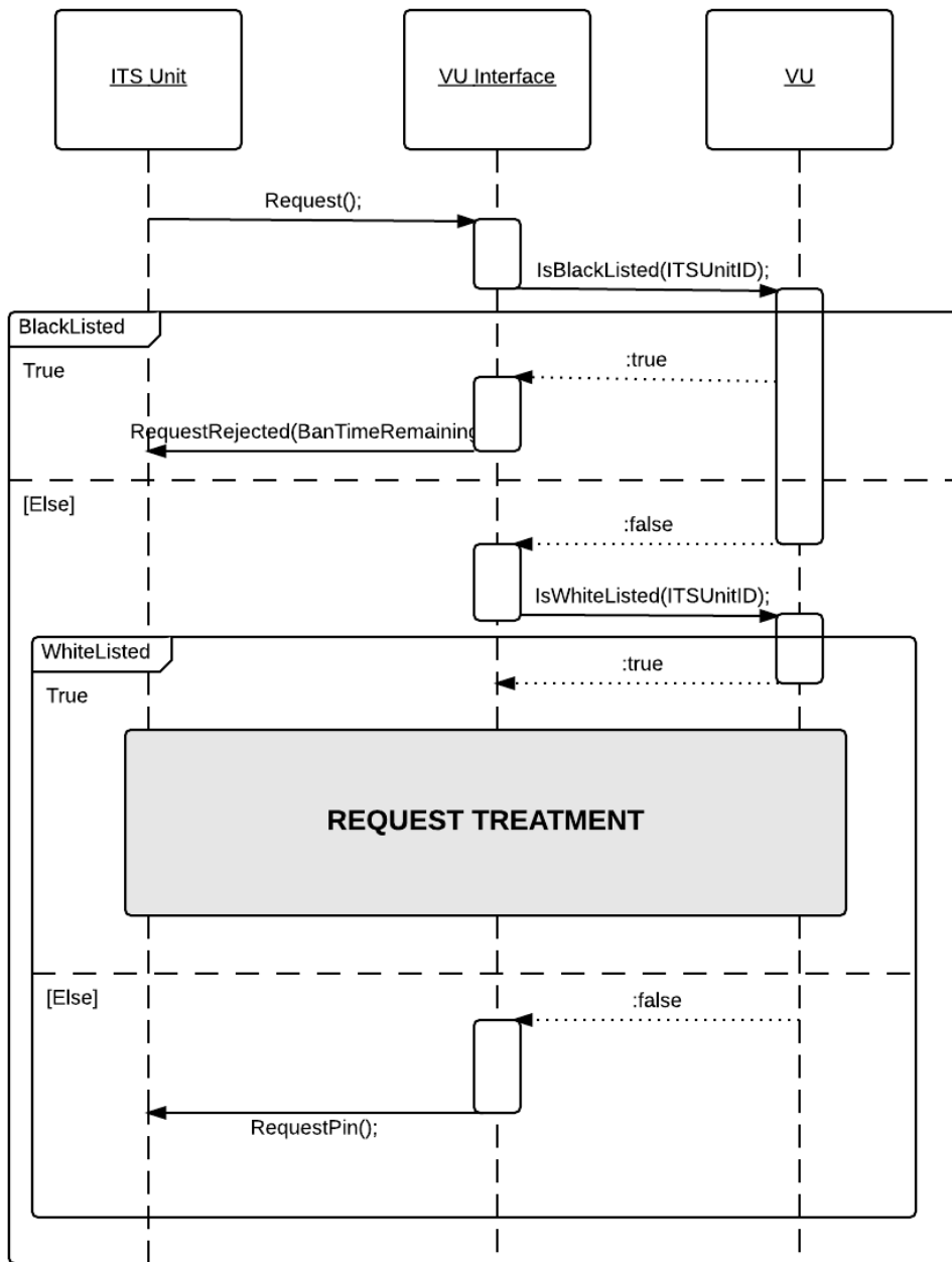
Figure 19. Sequence Diagram for ITS Unit's authorization verification
