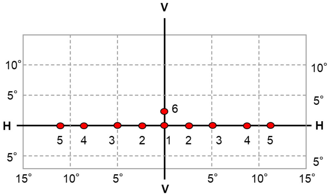
Figure A4-III Primary driving beam - position of test points
