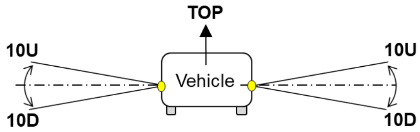
Figure A4-XIV Vertical geometric visibility for cornering lamps
