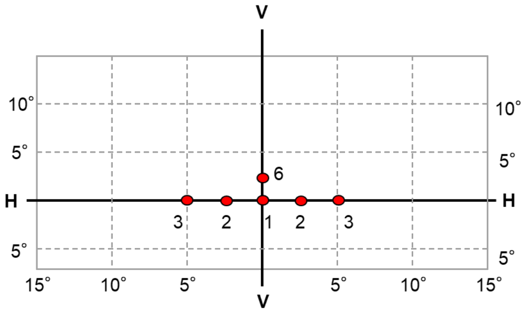
Figure A4-IV Secondary driving beam - position of test points
