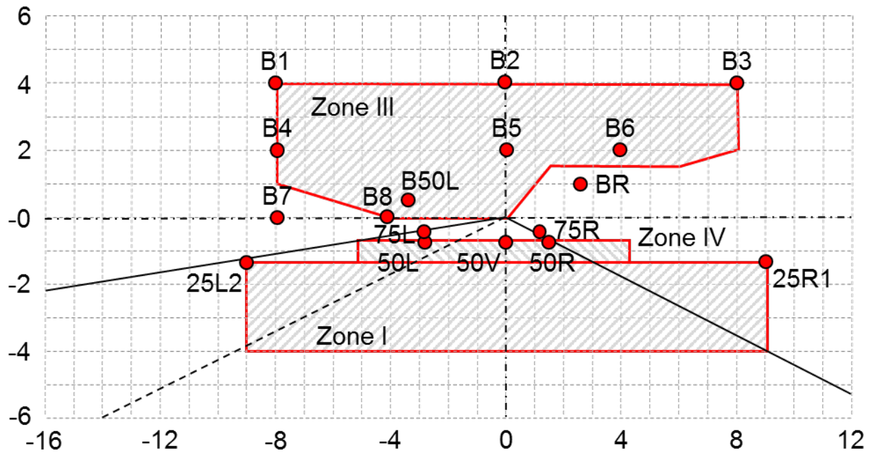
Figure A4-V Passing-beam for right-hand traffic
