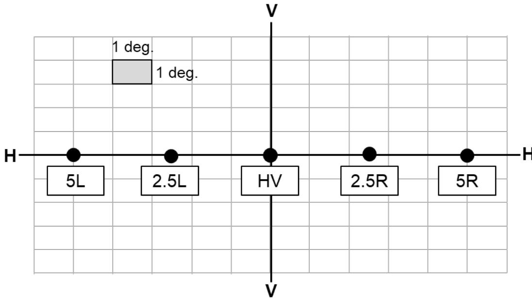
Figure A4-II Driving beam test points
