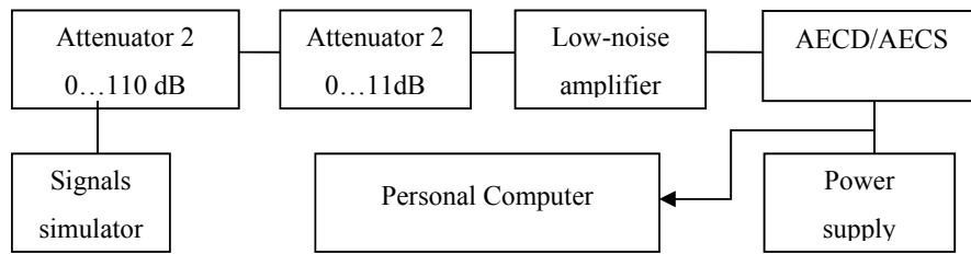
Figure 5 – Arrangement for evaluation of GNSS module sensitivity
