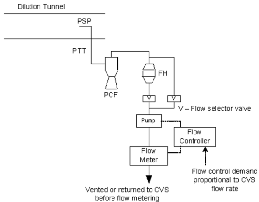
Figure A5/12 Particulate sampling system
