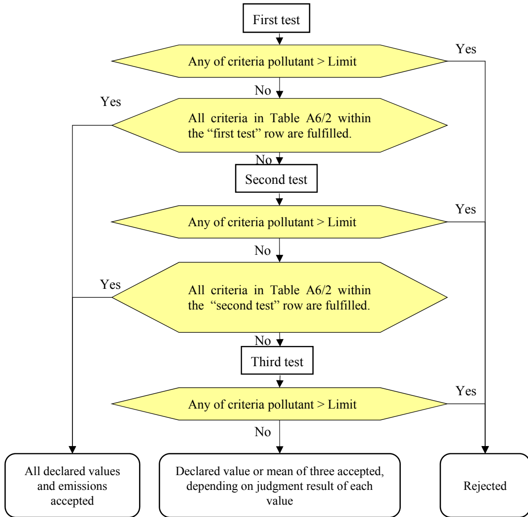
Flowchart for the number of Type 1 tests
