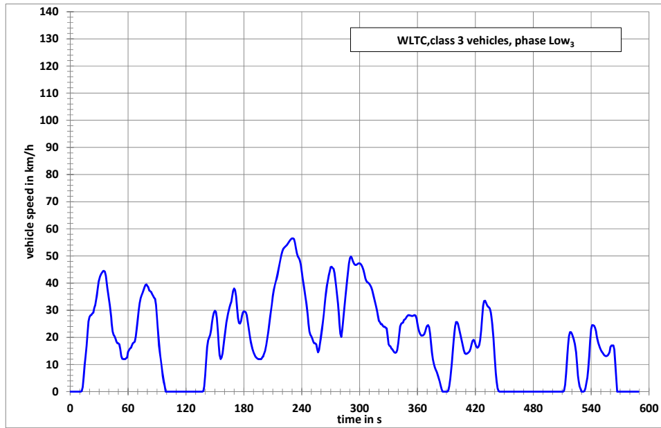
WLTC, Class 3 vehicles, phase Low 3
