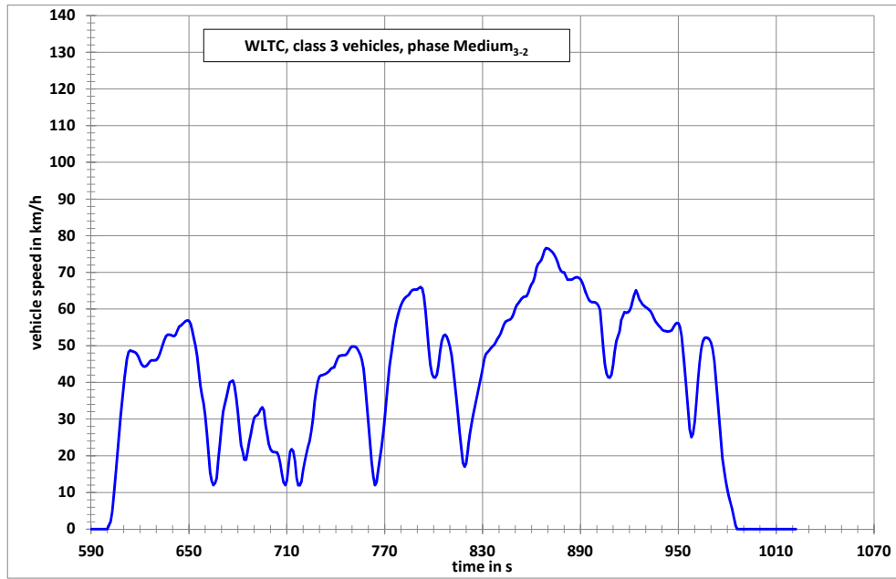
Figure A1/9 WLTC, Class 3 vehicles, phase Medium 3,2
