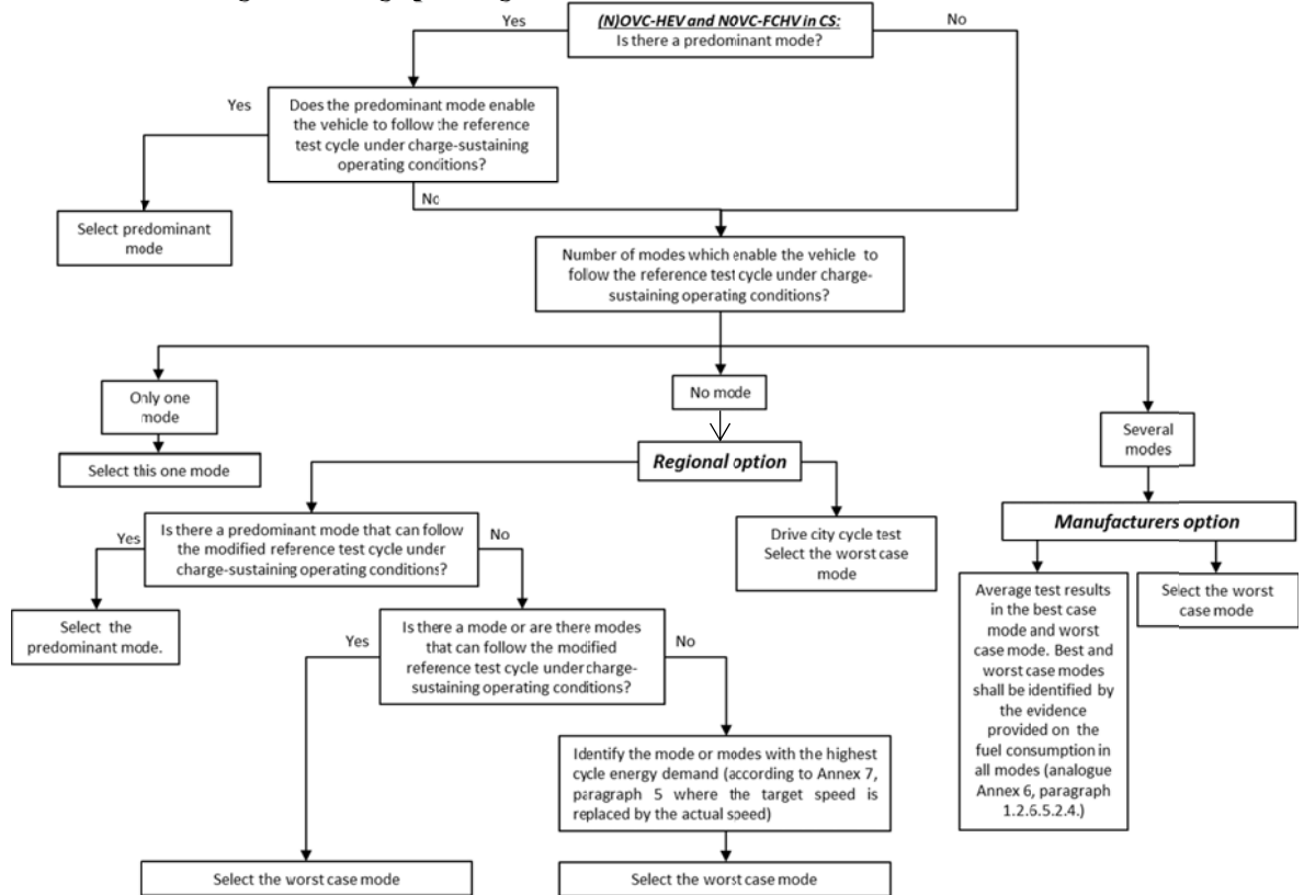
Figure A8.App6/2 Selection of a driver-selectable mode for OVC-HEVs, NOVC-HEVs and NOVC-FCHVs under charge-sustaining operating condition
