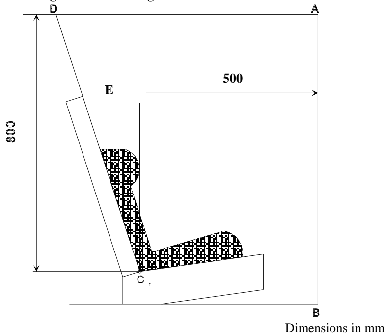
Arrangement for testing a forward-facing device
