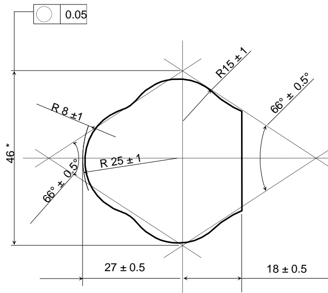
Figure 2 Stopping device olive-shaped knob
