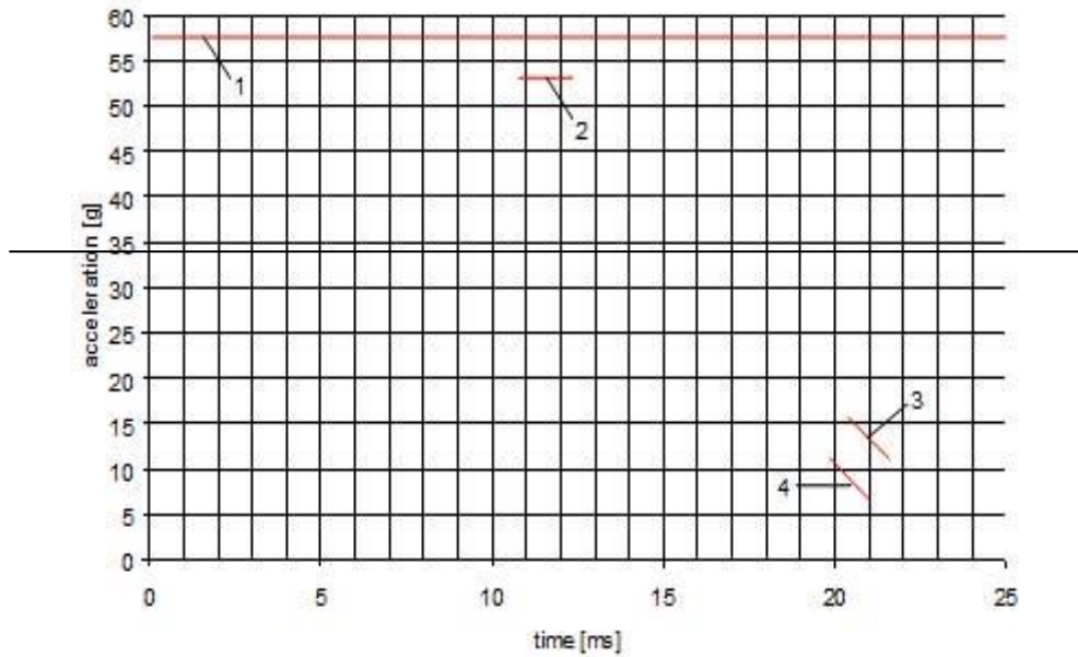
Figure 1 Corridor for the padding material
