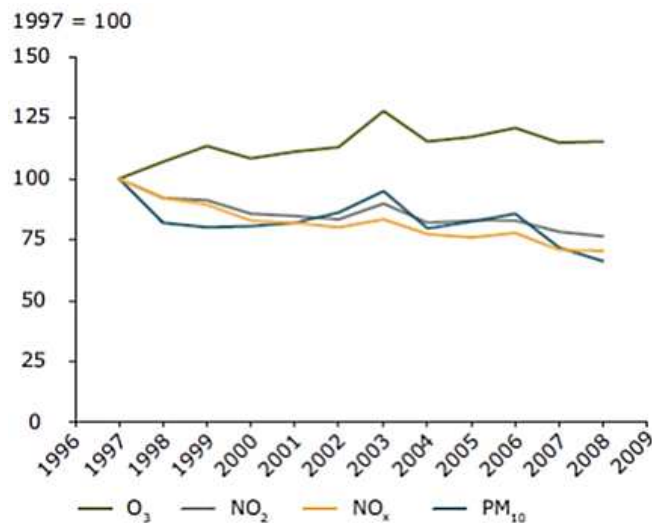
Figure 4. Indexed trends in air quality
