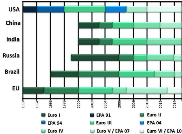
Figure 4. Passenger cars are getting cleaner worldwide
