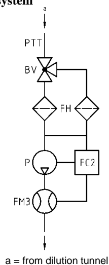
Figure 17 Scheme of double dilution particulate sampling system
