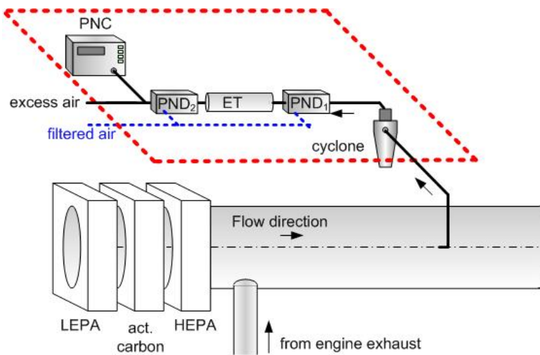
Figure 20 Schematic of Recommended Particle Sampling System – Full Flow Sampling
