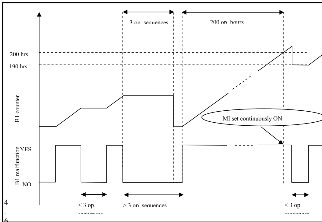
Figure C2 Illustration of the B1 counter activation principles
