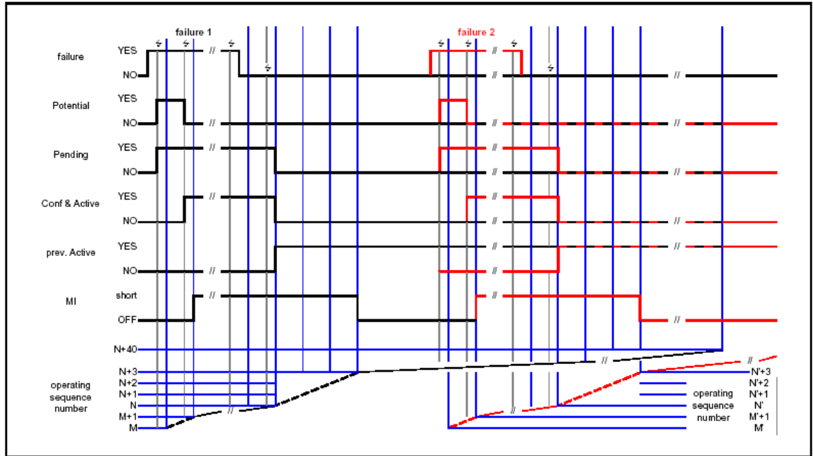
Figure 2 DTC status in case of 2 consecutive different class B1 malfunctions
