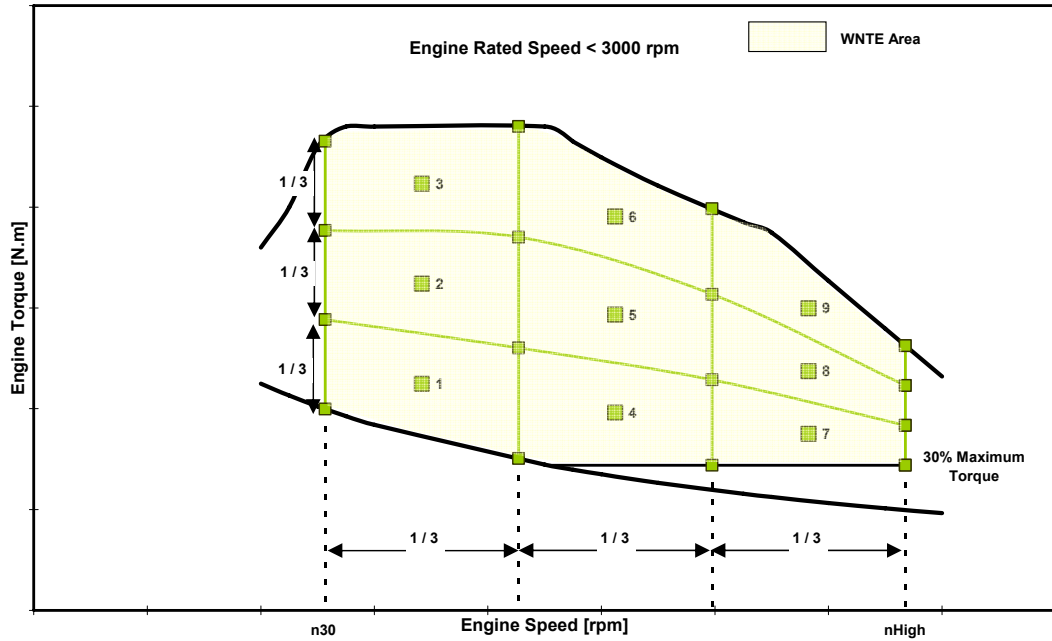
Figures 5 and 6 WNETE test cycle grids
