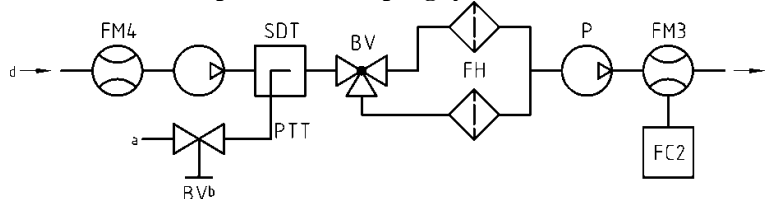
Figure 17 Scheme of double dilution particulate sampling system
