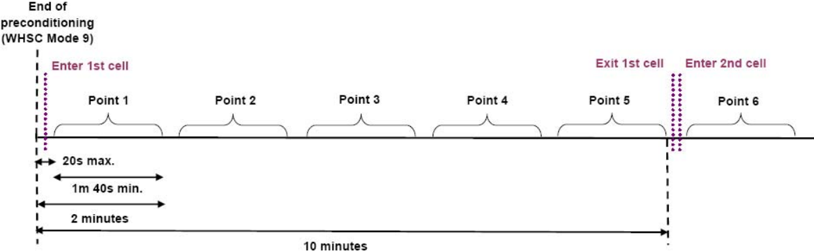
Figure 4 Schematic example of the start of the WNTe test cycle
