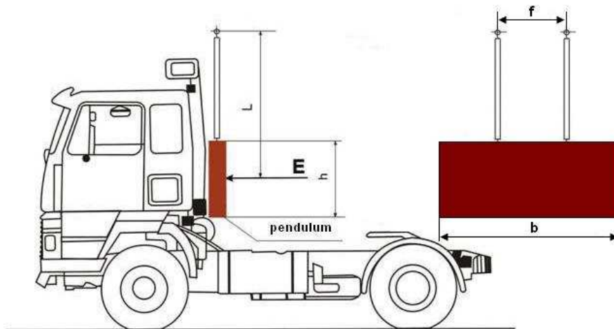
Fig. 4. – Rear-wall strength test
