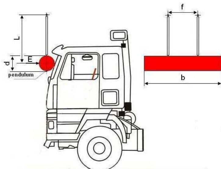
Fig. 2. – Front pillar impact test (Test B).
