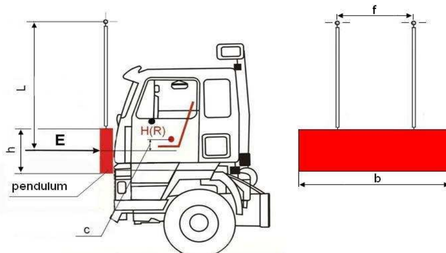
Fig. 1 – Front impact test (test A).
