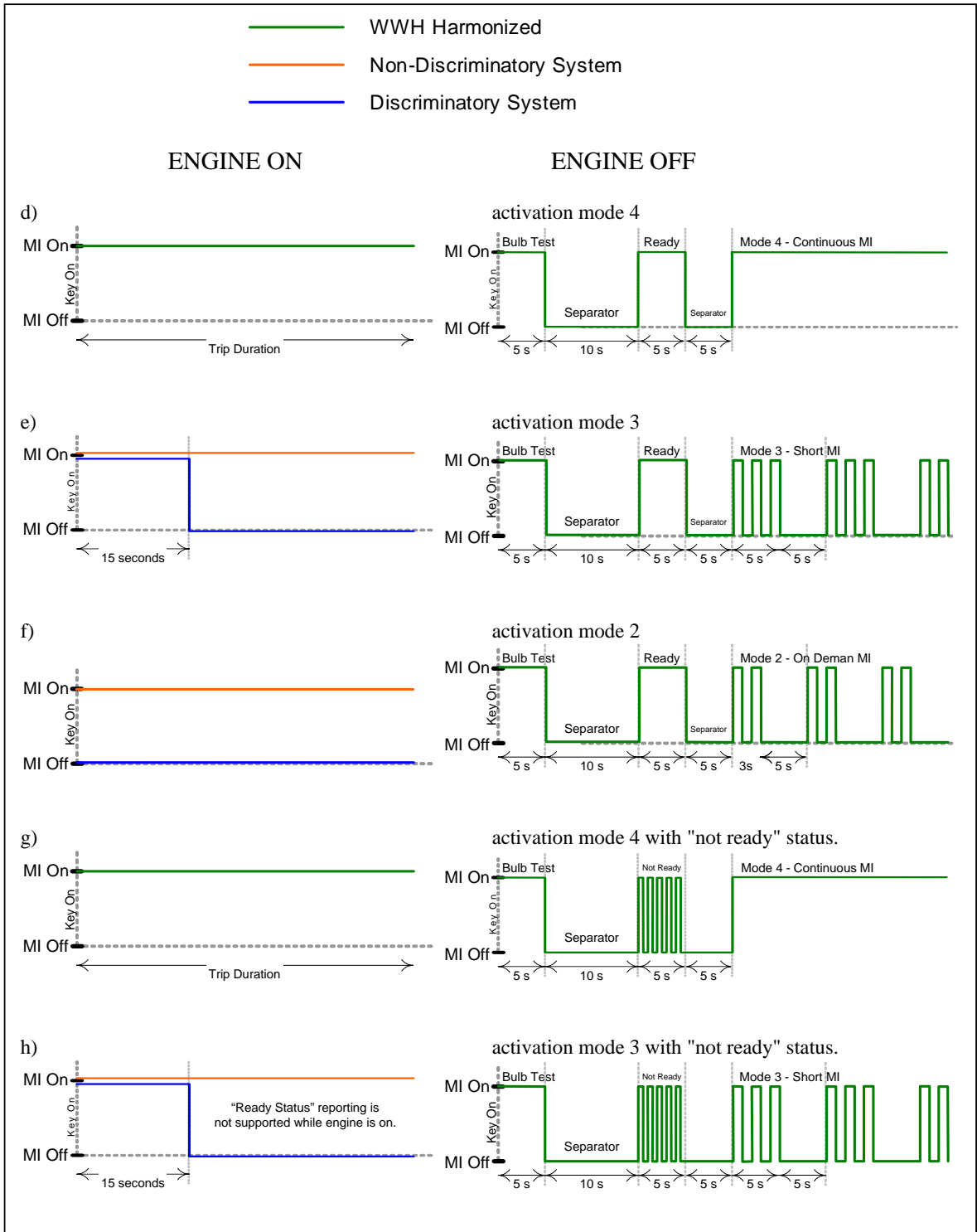
Figure B2: Malfunction display strategy
