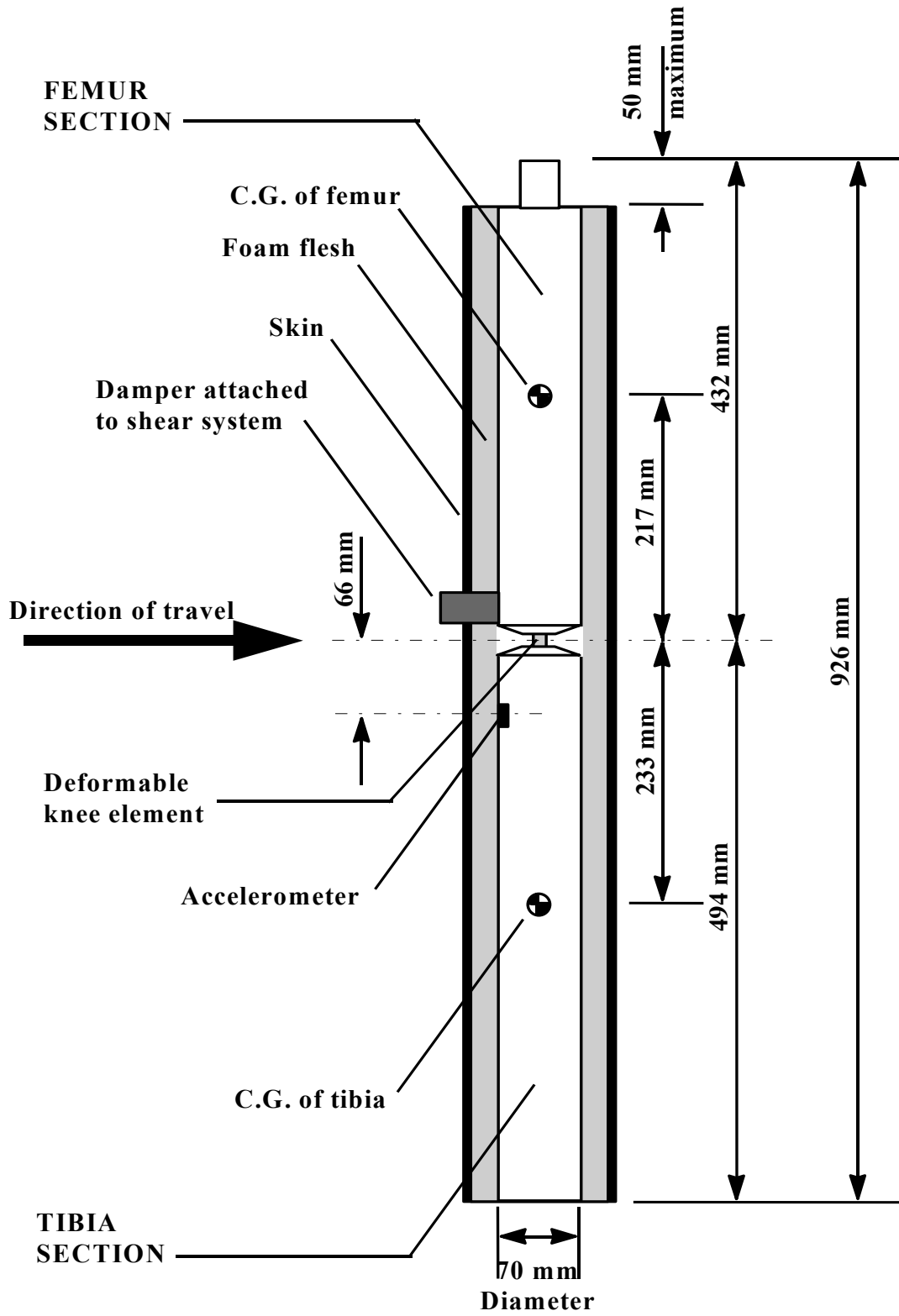
Figure 14: Lower legform impactor. (see §paragraph 6.3.1.1.)
