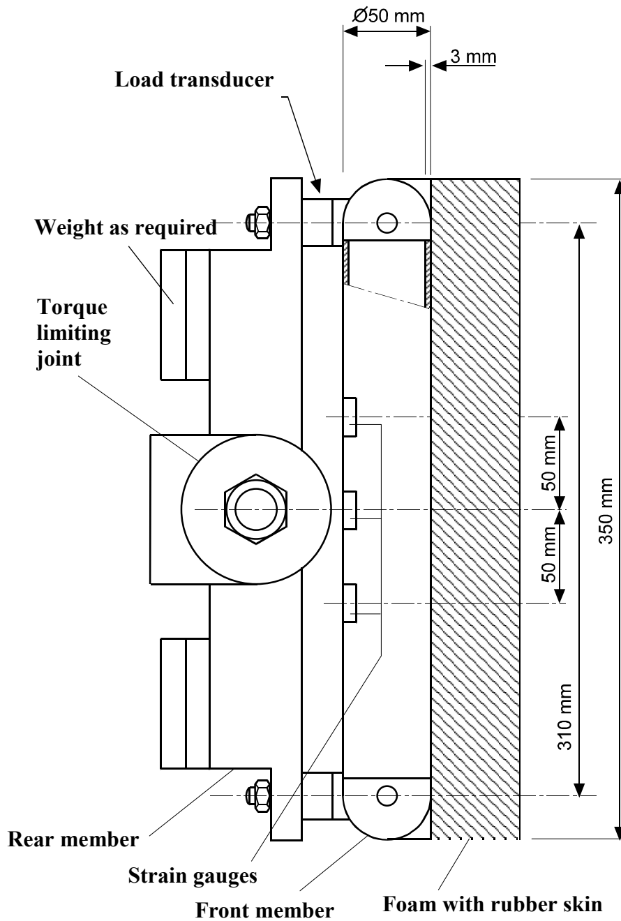
Figure 15: Upper legform impactor (see §paragraph 6.3.1.2.)
