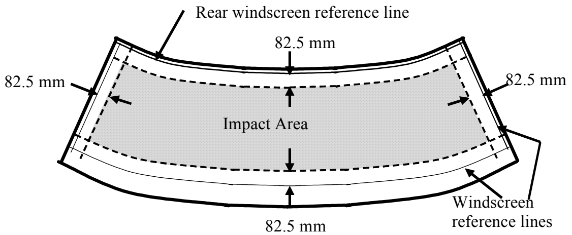
Figure 12: Windscreen test area: (see paragraph §3.34.)
