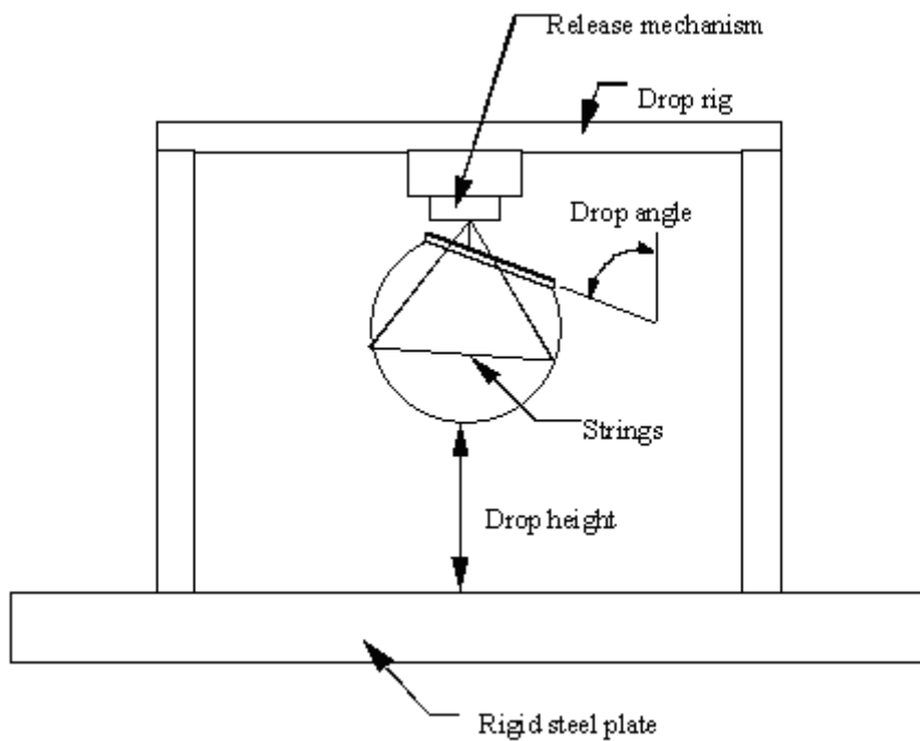
Figure 2728. Test set-up for dynamic headform impactor biofidelity test (see §paragraph 8.3.3.1.)
