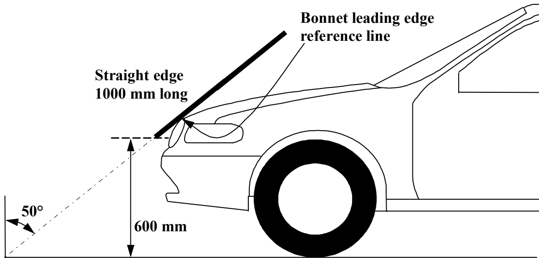
Figure 1: Bonnet Leading-leading Edge-edge Reference-reference Line line. (see §paragraph 3.5.)
