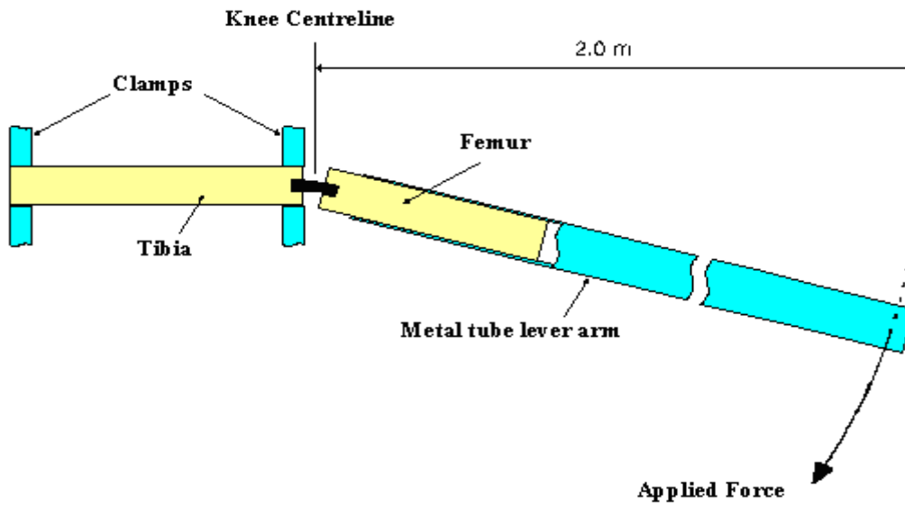
Figure 2223. Top View of Test set-up for static lower legform impactor bending certification test (see §paragraph 8.1.1.4.)
