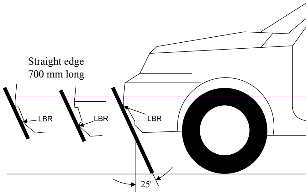
Figure 7: Lower Bumper-bumper Reference-reference Line line, LBRL- (see paragraph §3.19.)
