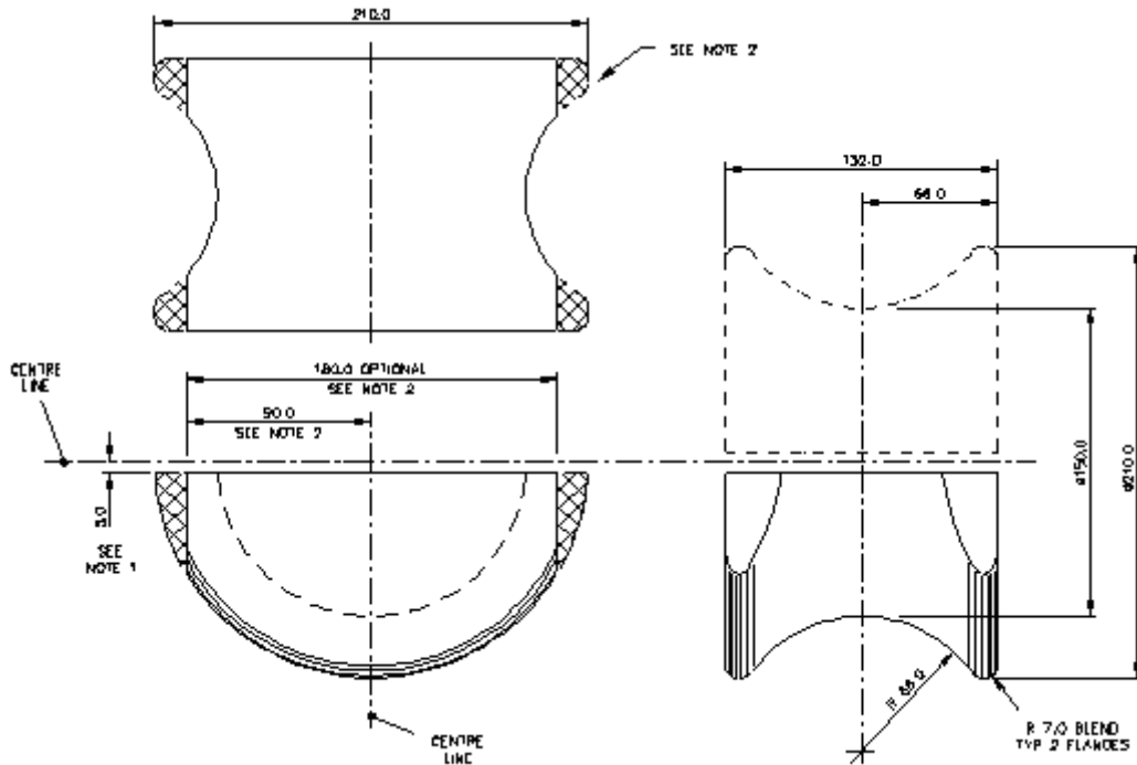
Figure 2526. Details of dynamic lower legform certification impactor face (see §paragraph- 8.1.2.4.2.)
