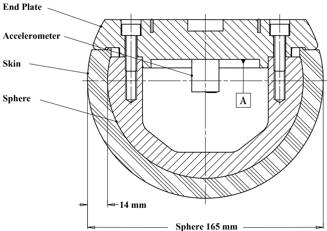
Figure 16: Child headform impactor (see §paragraph 6.3.2.1.)
