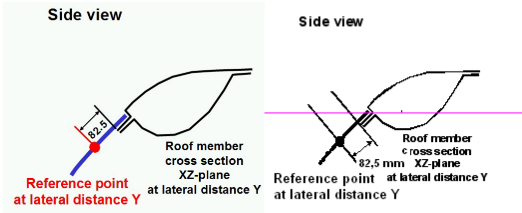
Figure 13a: Windscreen Rear-rear Reference-reference Line line (see paragraph §3.33.) This diagram needs to be changed to reflect definition.
