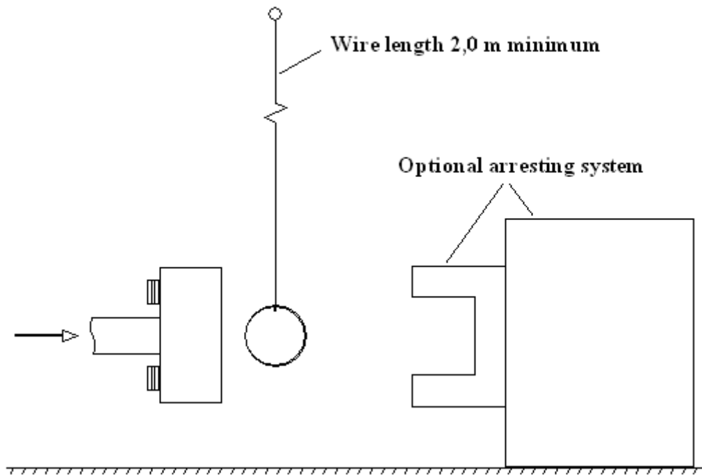
Figure 2627. Test set-up for dynamic upper legform impactor certification test (see §paragraph- 8.2.3.6)
