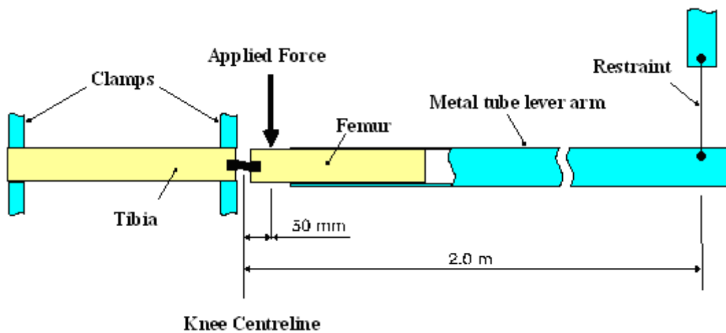
Figure 2324. Top View of Test set-up for static lower legform impactor shearing certification test (see §paragraph 8.1.1.5.)
