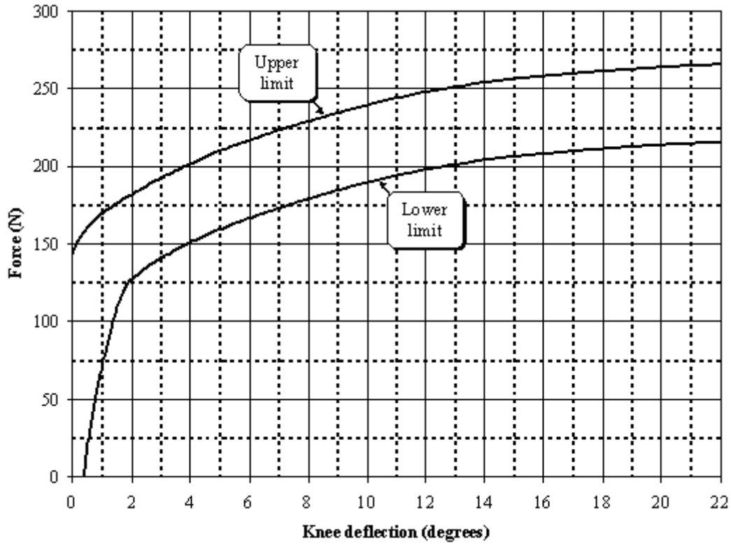
Figure 2021. Force versus angle requirement in static lower legform impactor bending certification test (see §paragraph 8.1.1.2.)
